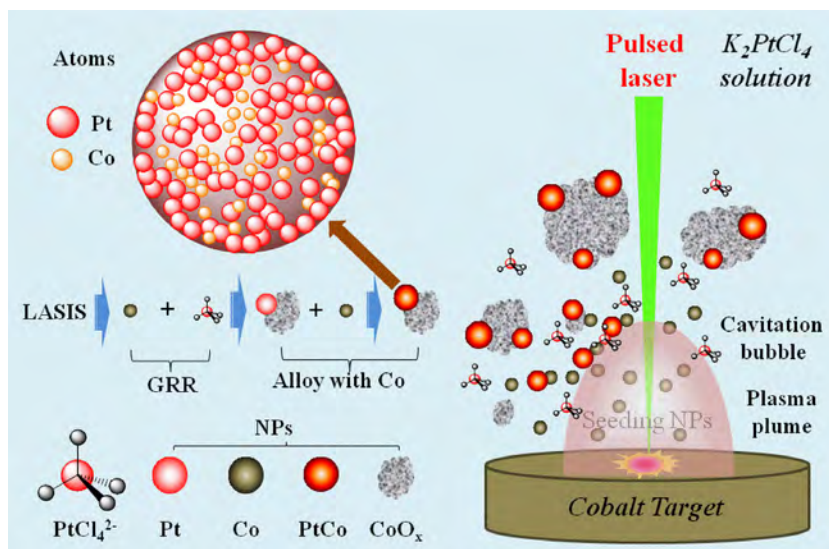
Fig. 1. Schematic representation of the tandem LASIS-GRR technique that synthesize PtCo/Co x nanocomposites (NCs).
