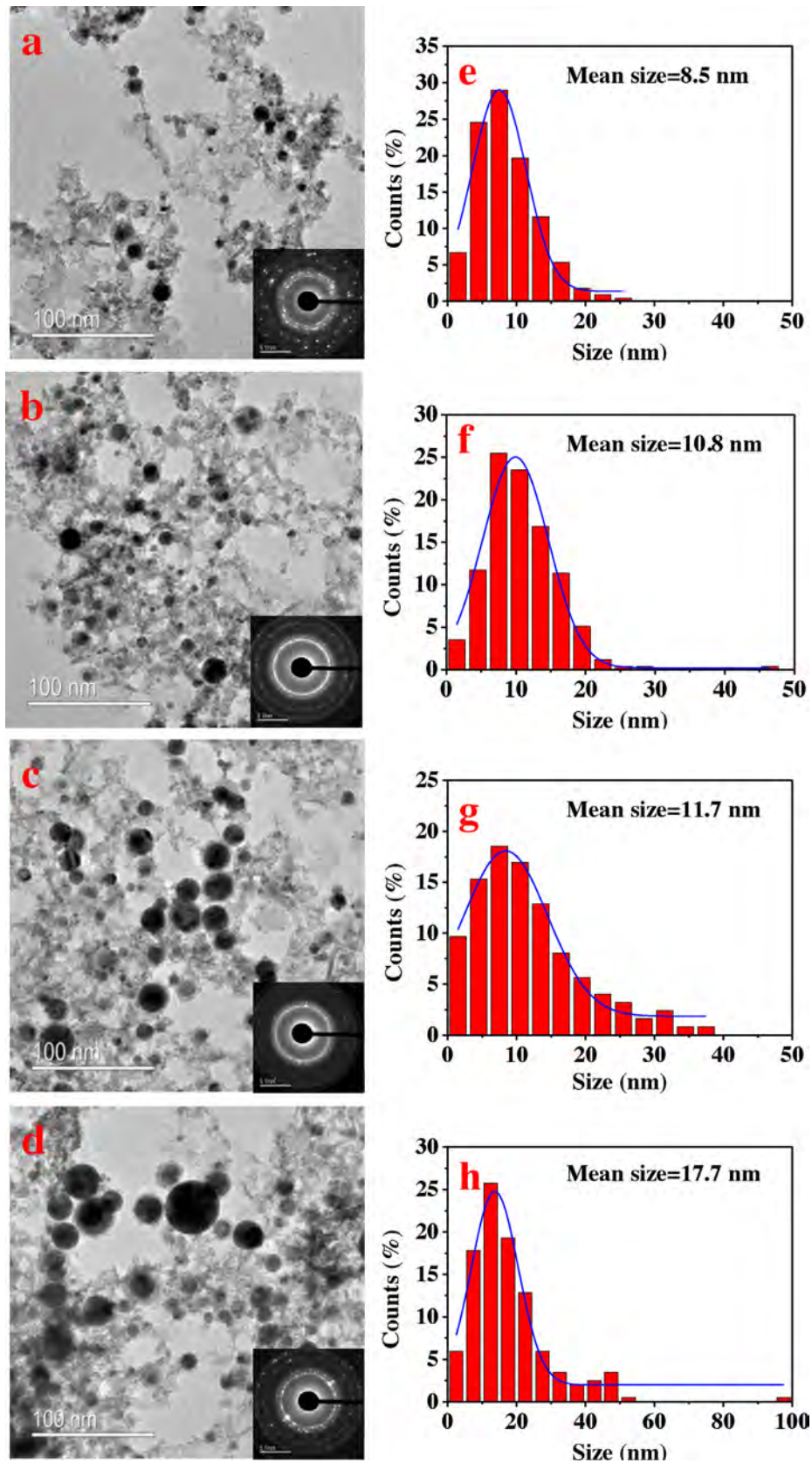
Fig. 2. (a–d) TEM images (Magnification: 80K) along with the corresponding SAED patterns (inset) for the PtCo/CoO x NPs synthesized by LASIS–GRR using different Pt:Co atomic ratios of: (a) 1:9 (PtCo-1); (b) 1:4 (PtCo-2); (c) 1:2 (PtCo-3); (d) 1:1 (PtCo-4). The scale bar in for SAED patterns is 5 (1/nm); (e–h) Corresponding size distributions for dark colored PtCo alloyed NPs in a–d.
