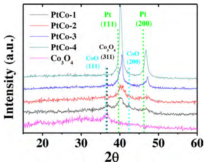
Fig. 5. Comparison of XRD patterns for PtCo/Co x nanocomposites with different Pt:Co ratios along with standard peak positions for Co 3 O 4 , CoO and Pt indicated by black, blue and green vertical lines respectively.
