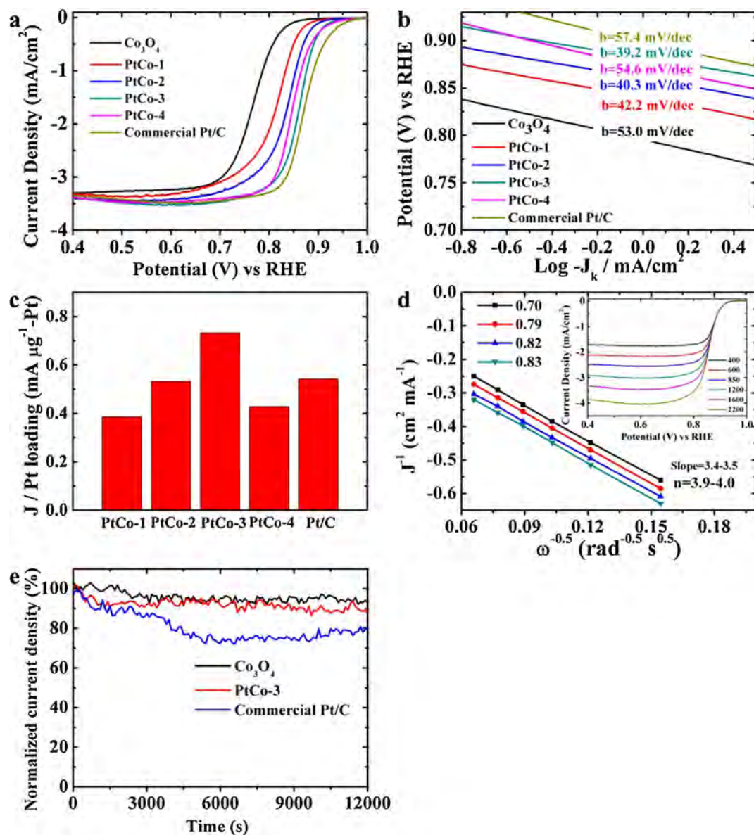
Fig. 6. Electrochemistry data for as-synthesized \text{Co}_3\text{O}_4 NPs and PtCo/Co _x NCs compared to standard Pt/C samples using: (a) Linear sweep voltammograms for ORR analysis in 1 M KOH electrolyte saturated with dissolved \text{O}_2 at 1600 rpm and scan rate of 5 mV/s; (b) Tafel plots from a; (c) Comparison of mass activities per unit Pt mass loading at 0.85 V vs. RHE; (d) Koutecky–Levich plots from rotating disk voltammogram (RDV) data (shown in inset) for PtCo-3 at different potentials (0.70–0.83 V) indicate four electron transport process for ORR; (e) Stability comparison for \text{Co}_3\text{O}_4 , PtCo-3 and standard Pt/C through chronoamperometry (CA) tests.
